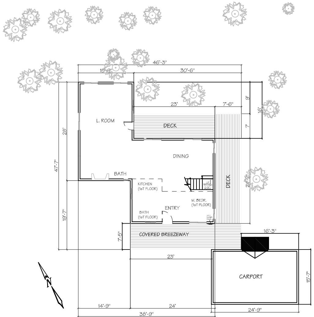
(E) FLOOR PLAN
